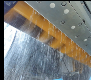
Horizontally screw conveyor wash system
