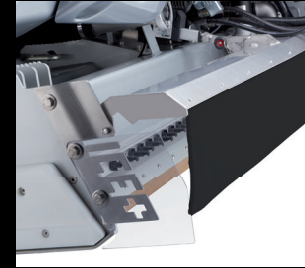
ICEplus Flexi Water spraying system + electrically powered cloth support
